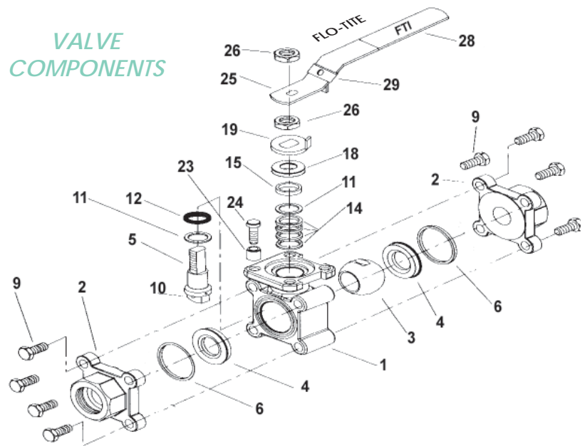
Exploded View For 1/4"~2-1/2"
